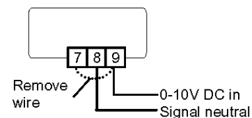
Abb 8: Externes Regelsignal
